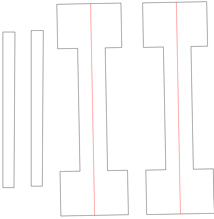
AIRFOIL SPACERS
